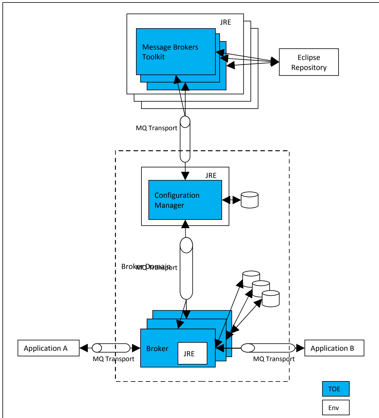
Figure 1 – WMB Components
